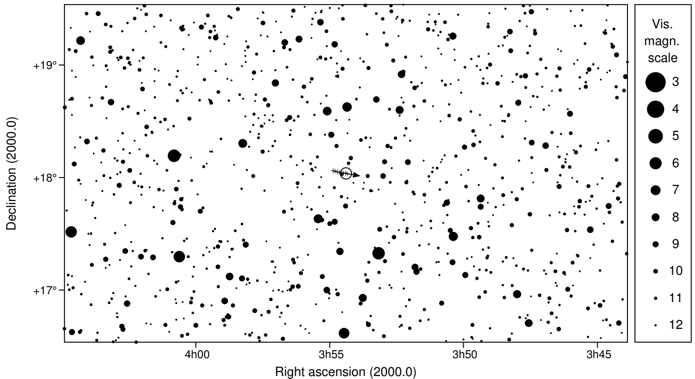
5h17m00s – 5h27m00s; int. 1m
