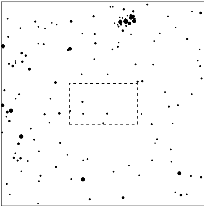
5h17m00s – 5h27m00s; int. 1m
